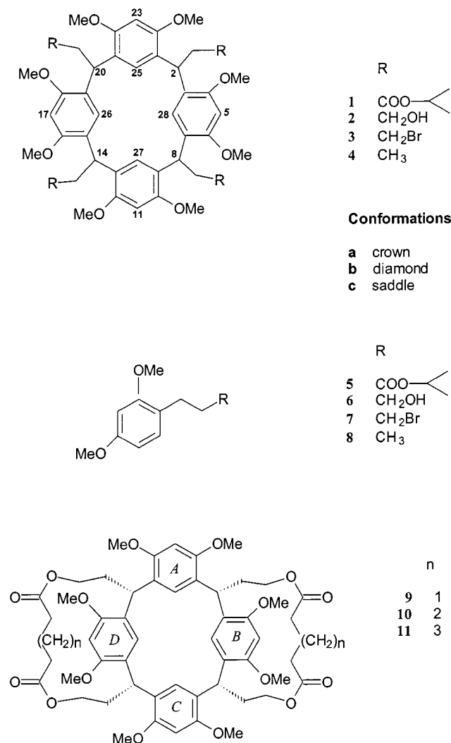
Figure 1. Resorcin[4]arene derivatives and monomer models synthesized
