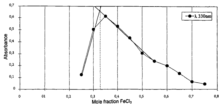
Figure 3. Stoichiometry of complex 1a / \text{FeCl}_3 calculated according to the Job method at \lambda = 330 \text{ nm} in the UV/Vis spectrum
